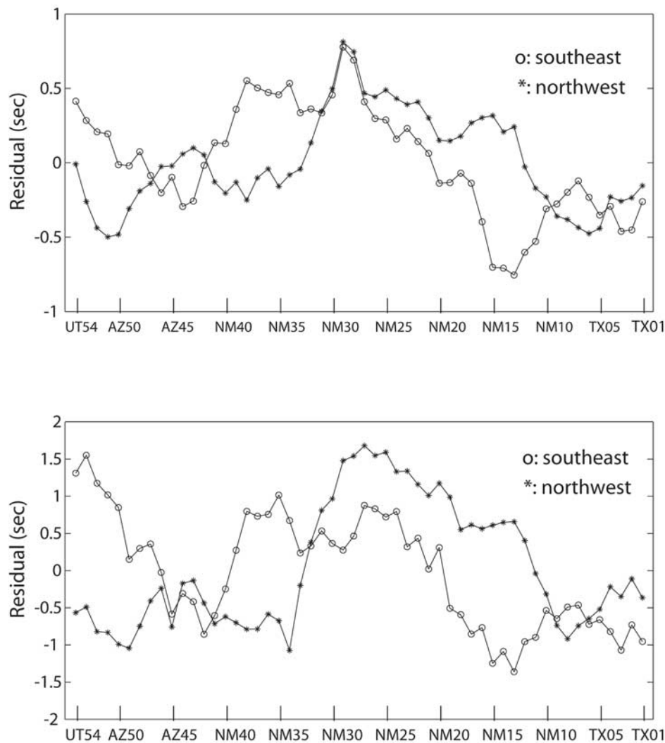
Figure 5. Average corrected P and S residuals as a function of back azimuth for La Ristra stations. The open circles are average residuals from earthquakes to the southeast of the array and stars are residuals from earthquakes to the northwest of the line.
