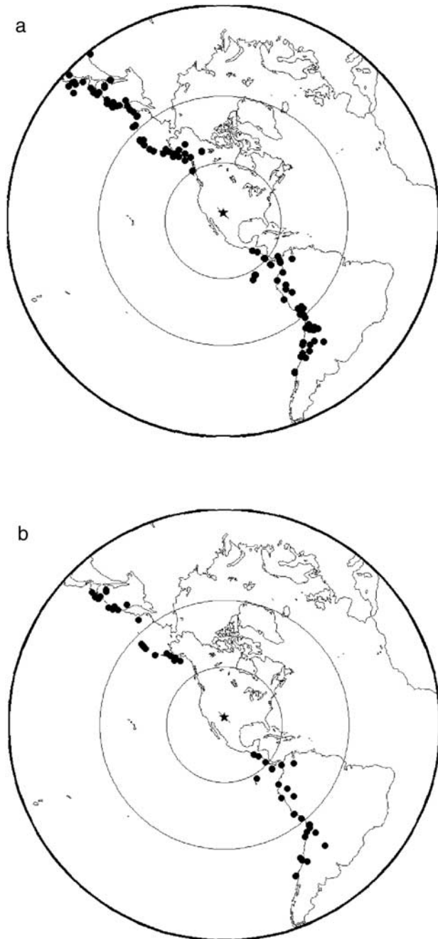
Figure 2. Map showing the earthquakes used in the tomographic inversion. Figure 2a shows the events used that produced clear P waves and Figure 2b shows the events used that produced clear S waves. The star in the center of Figures 2a and 2b shows the La Ristra array. Not shown are a few earthquakes at distances beyond 100^\circ that were used to measure SKS wave travel times.
