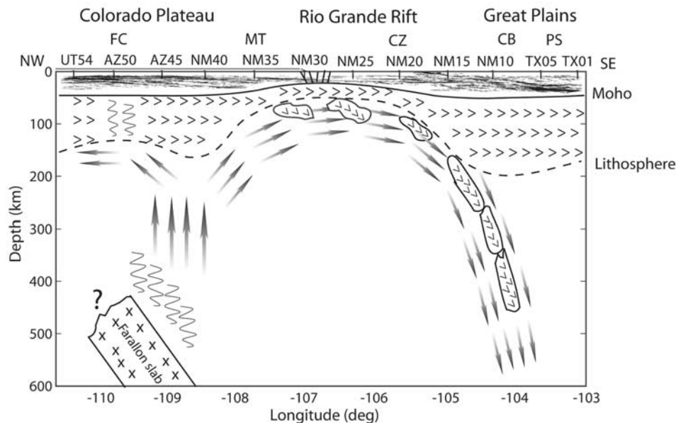
Figure 9. Schematic illustration of our interpretation of present-day mantle structure beneath the Rio Grande rift and surrounding regions. The full three dimensional flow of mantle in the region is unknown but we indicate certain features projected onto the two-dimensional plane beneath the RISTRA line that are indicated by the tomography results. The stippled pattern in the shallow mantle indicates lithosphere. Arrows indicate mantle flow direction and wavy lines indicate mantle enriched in volatiles. Volatiles released from the Farallon plate are entrained in mantle upwelling eventually rising under Mount Taylor. Downwelling is occurring under the Great Plains. In our model a significant portion of the lithosphere from Mount Taylor to Carrizozo has been removed and is entrained in the eastern downwelling. FC is the Four Corners region, MT is Mount Taylor, CZ is Carrizozo, CB is Carlsbad, NM, and PS is Pecos, TX.
