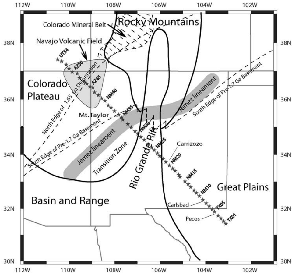
Figure 1. Map of the southwestern United States showing the location of the La Ristra array seismic stations. The location of the main physiographic and tectonic provinces discussed in the text, are also shown. Dashed lines show boundaries of two Proterozoic provinces from Karlstrom and Humphreys [1998]. The Colorado mineral belt lies along the northwestern Proterozoic boundary shown in the figure passing through Aspen.
