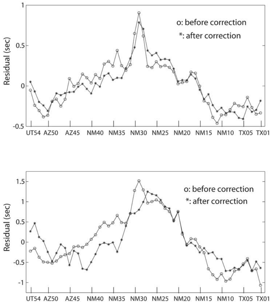
Figure 4. Average P and S residuals at each station in the La Ristra array (open symbols). The closed symbols show the average residuals corrected for topography, crustal velocity variations, and Moho depth.
