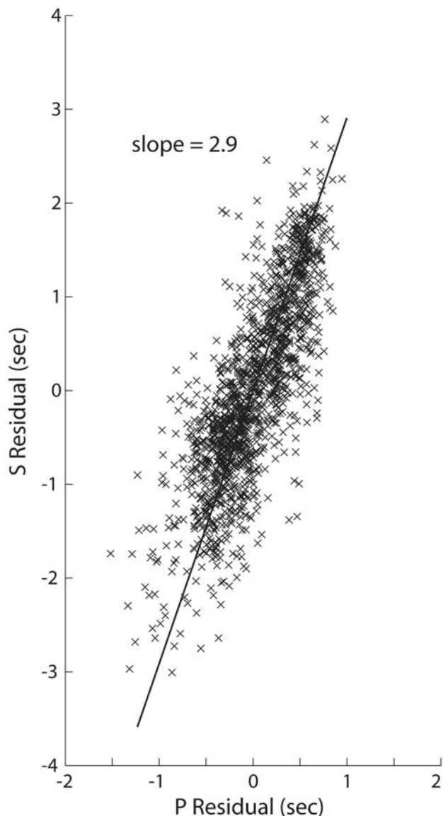
Figure 8. Plot of travel time residual of P versus S for common earthquakes and stations. The least squares fit line through the data has a slope of 2.9.
