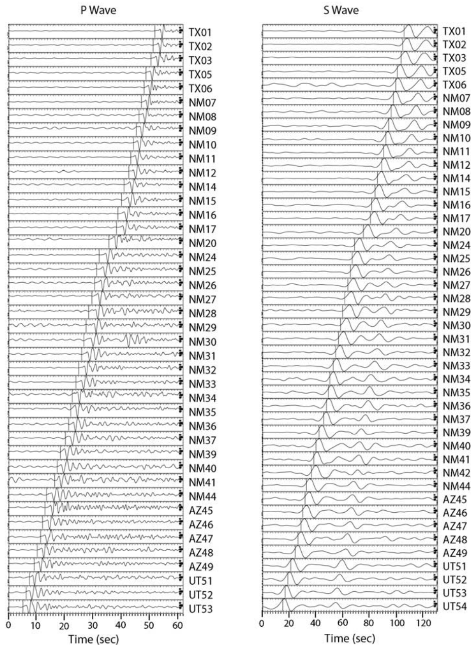
Figure 3. Example of P and S data recorded by La Ristra stations from a single earthquake. Predicted origin times are marked on the data. Note the similarity in waveform at the beginning of the P and S waves and the variations in arrival time with respect to the predicted times.
