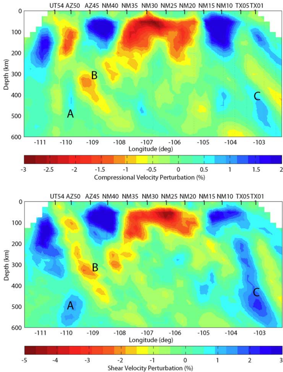
Figure 7. The P and S models obtained through inversion of travel time residuals.
