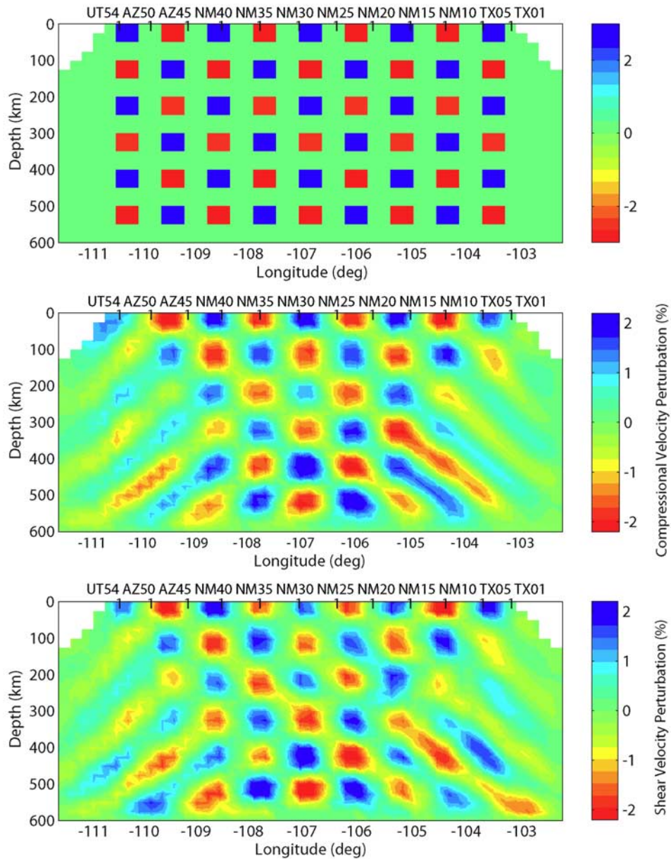
Figure 6. Synthetic resolution test. The top panel shows an input structure used for P and S velocity. The model consists of blocks of 50 km dimension used to compute a synthetic data set. The lower two panels show the result of inverting the synthetic P and S data, respectively, using the same smoothing and algorithm applied to the real data.
